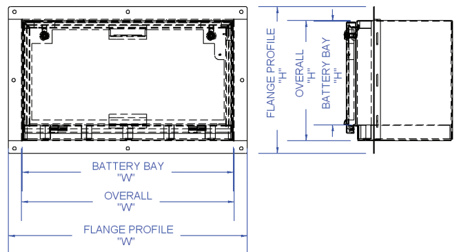
WALL 4WHAZ
